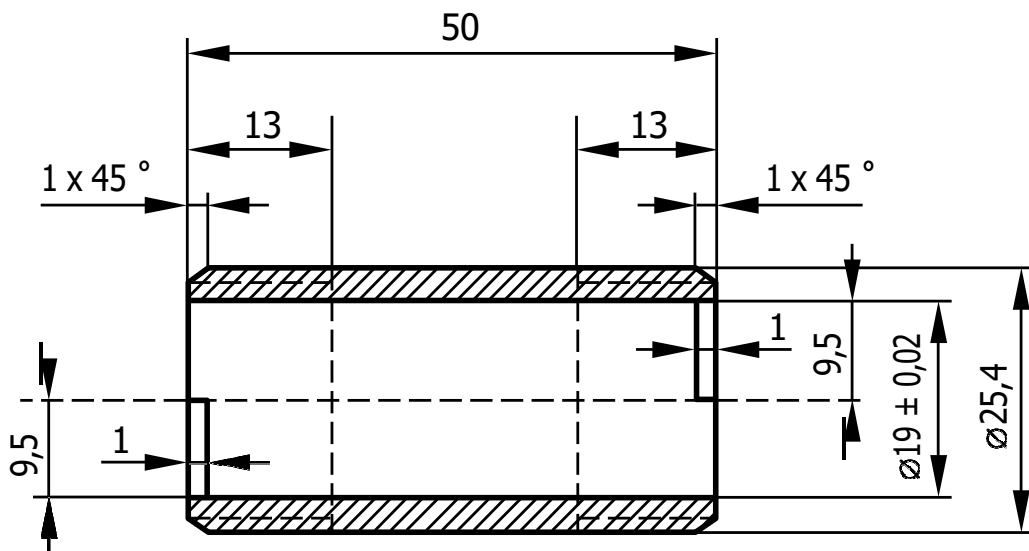
Figure K.5 — Item 3 - Mixing tube
