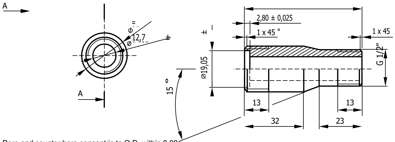
Figure K.11 — Item 9 - Inlet
